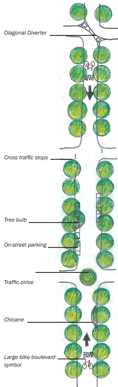
Figure 2.9: Bicycle Boulevard
